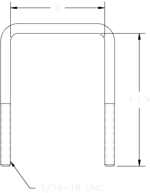
SQUARE U-BOLT
